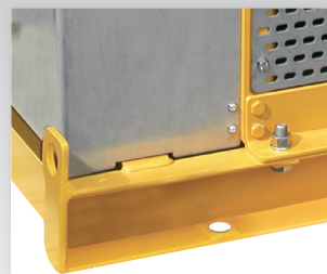
Offshore paint with sandblasting and carbozinc primer
